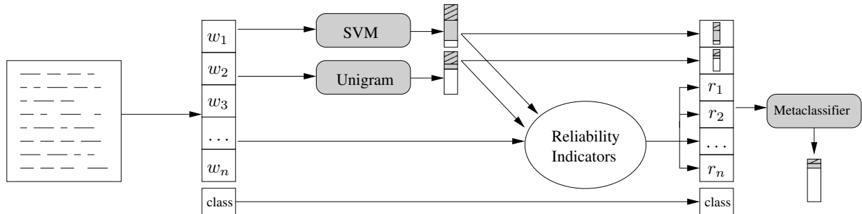
Figure 4: Architecture of STRIVE . In STRIVE , an additional layer of learning is added where the metaclassifier can use the context established by the reliability indicators and the output of the base classifiers to make an improved decision. The reliability indicators are functions of the document and/or the output of the base classifiers.
